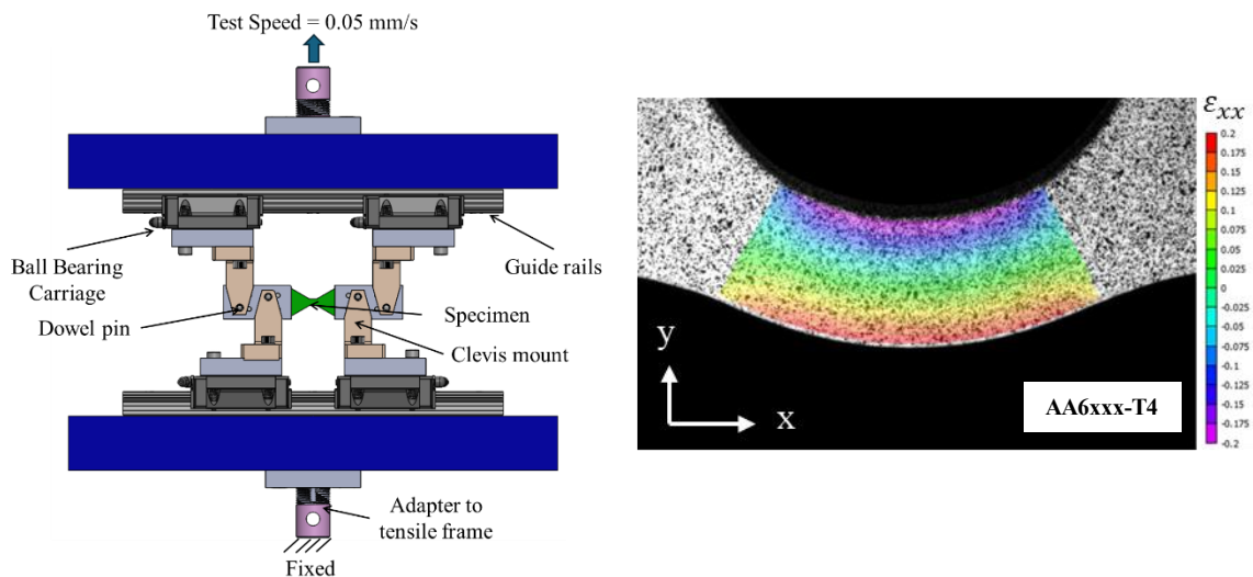
Figure 1: Design of the in-plane bending test (left), and resulting strain distribution in the sample (right) measured using Digital Image Correlation (DIC).
