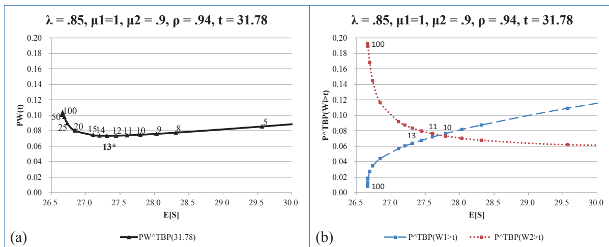
Figure 6 Trade-off curves corresponding to excessive wait probabilities of 10% (under nonidling policy). Nonidling policy corresponds to the left-most point on each curve.
