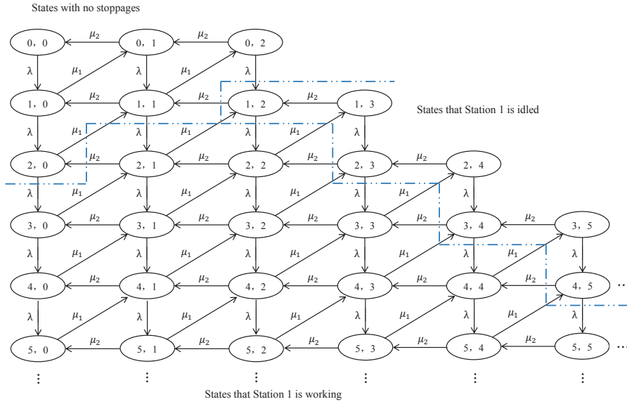
Figure 3 The MC (Q_1, Q_2) for TH = 1 .
