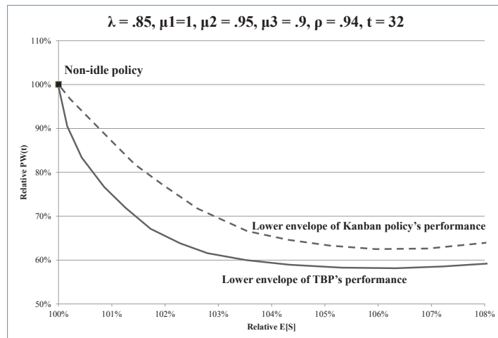
Figure EC.1 The lower envelope of the TBP's and Kanban policy's performances.
