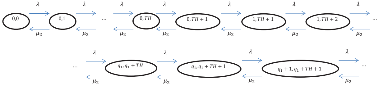
Figure 1 MC when \mu_1 = \infty and TH > 0 .
