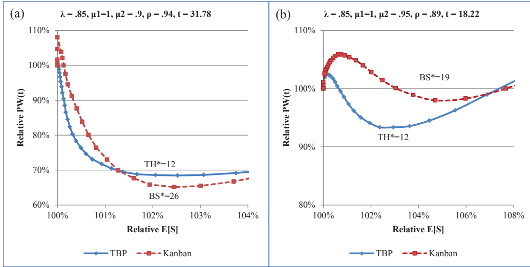
Figure 9 Trade-off curves corresponding to t = 31.78 under the TBP and the Kanban policy.
