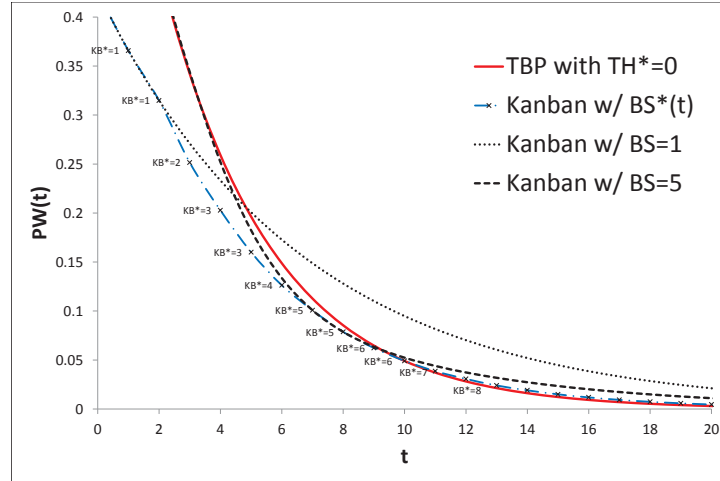
Figure 2 PW(t) as a function of t under TBP versus Kanban policy.
