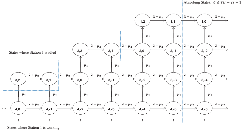
Figure 4 The revised TCMC (s, \delta) , when TH = 1 .
