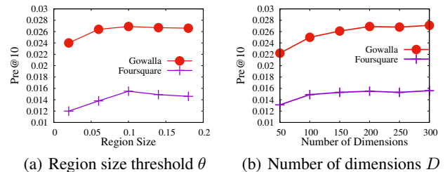
Figure 5: Effect of parameters.
