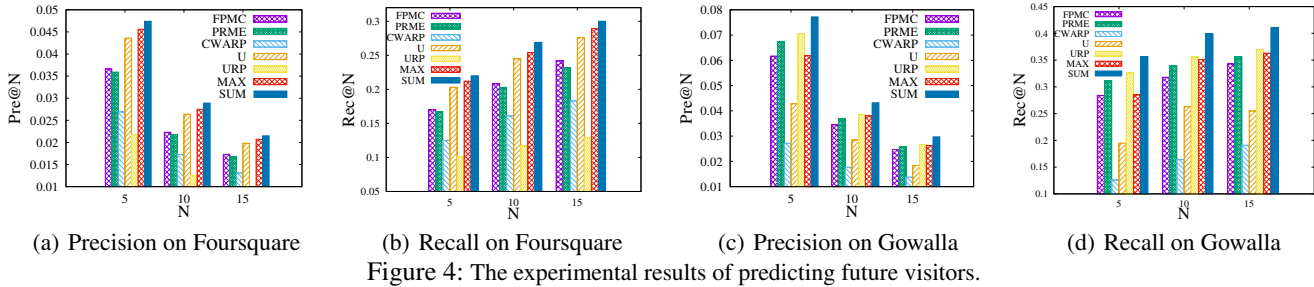
Figure 4: The experimental results of predicting future visitors.
