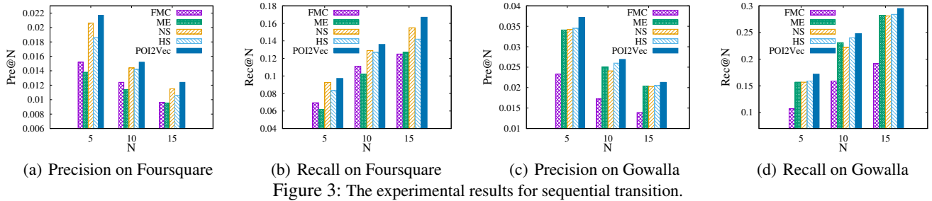
Figure 3: The experimental results for sequential transition.
