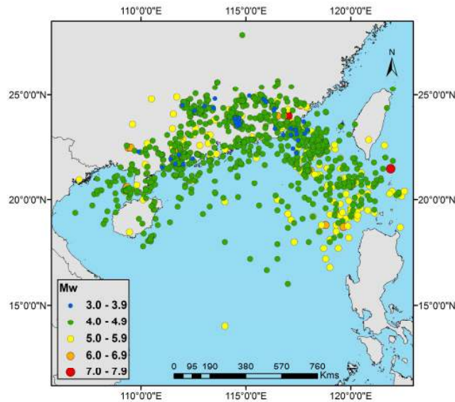
Figure 4. Historical earthquakes collected. The empirical relationships proposed by Wells and Coppersmith (1994) were used to convert the different magnitude types (i.e., M_s , and M_L ) into M_w .
