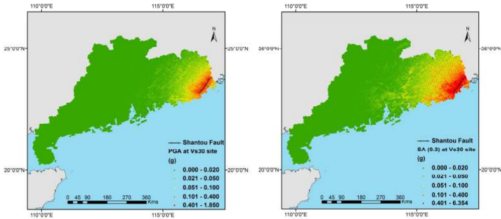
Figure 6. Generated surface (a) PGA and (b) S_a(0.3s) maps considering site conditions of Guangdong Province for the 1918 Shantou ( M_w=7.3 ) Earthquake.
