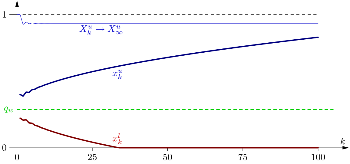
(b) \rho = 1, c = 3/2
