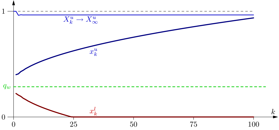
(a) \rho = 1/2, c = 3/2
