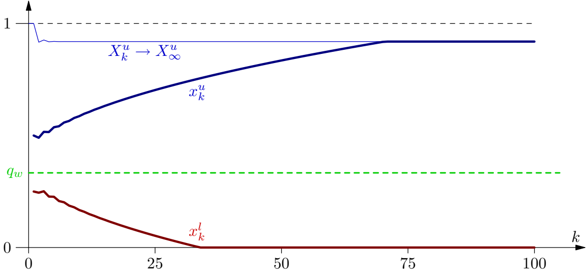
(c) \rho = 1/2, c = 1
