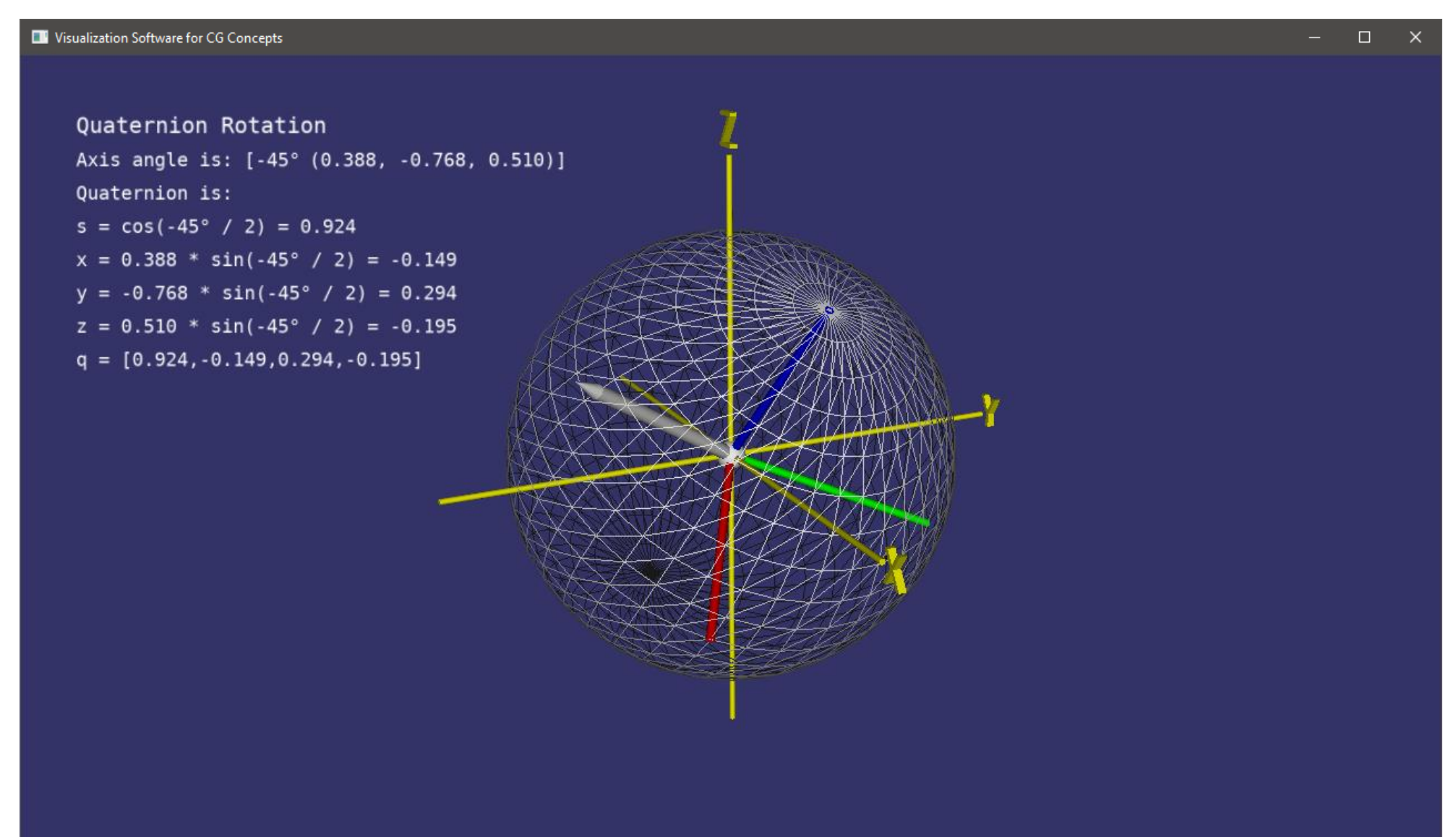
Quaternion Representation
