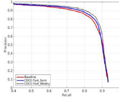
Figure 5: Comparison of character detection performance on ICDAR 2013 test dataset under different learning schemes from COCO-Text dataset. Baseline detector is trained only on ICDAR 2013 training dataset with character boxes. “COCO-Text_Semi” and “COCO-Text_Weakly” detectors are trained without annotation and with text block bounding boxes as described in Section 3.3.1 and Section 3.3.2, respectively.
