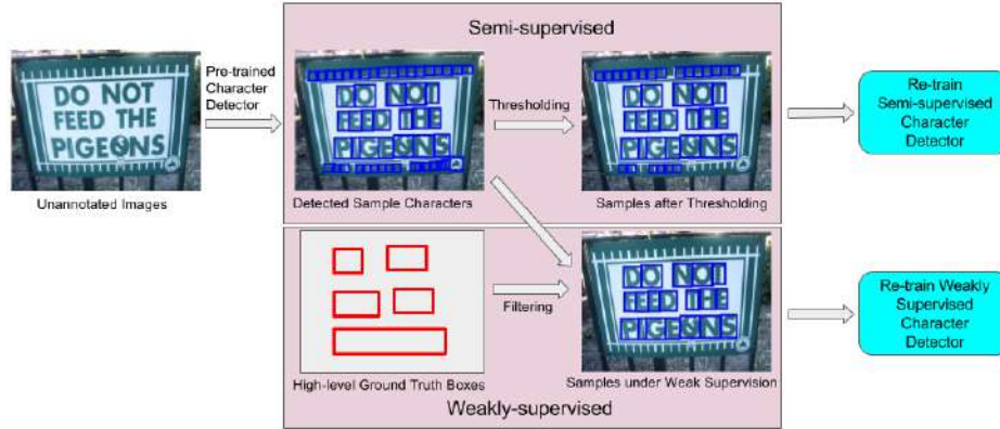
Figure 2: The framework of the proposed WeText system: A “light” supervised model is pre-trained using a small amount of annotated character image set. The light model is then applied to an unannotated dataset to search for more character samples which are combined with the small annotated dataset to train a semi-supervised model. Under certain weak annotations, better character samples can be searched to train a semi-supervised model.
