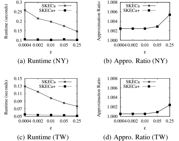
Figure 14: Varying \epsilon
