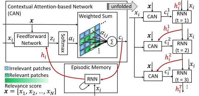
Figure 2. An illustration of our Episodic CAMN including its contextual attention-based network, the episodic recurrent memory and the feedback. The model consists of two major components: (1) the CAN adaptively selects the relevant context to contextualize the reference patch representation ( \mathbf{x}_i ); (2) the episodic memory summarizes the activated context in the past. The feedback from the episodic memory enables the CAN to iteratively refine the selected context over multiple iterations.
