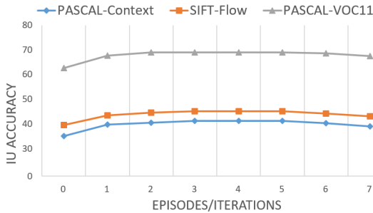
Figure 6. IU performance changes in terms of iterations.
