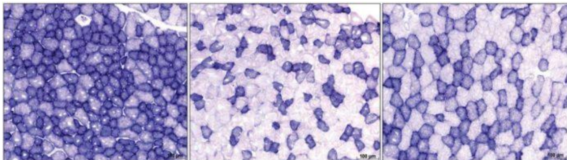
Microscopic images of the amount of enzyme activity (dark purple specks) in the mitochondria in the muscle of mice. When microbes were transplanted into germ-free mice, enzyme activity increased, which translates to a higher capacity for the muscle to produce energy. L-R: Muscle of standard laboratory mice, Muscle of germ-free mice, Muscle of germ-free mice transplanted with gut microbes from lab mice. CREDIT – NTU Singapore
