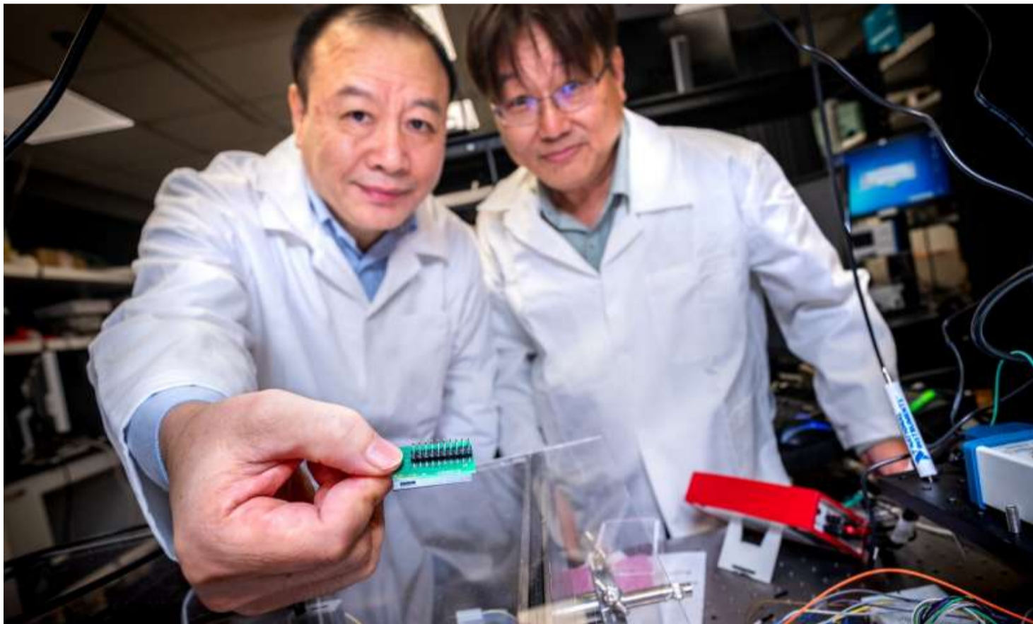
(L-R) NTU Prof Liu Ai Qun and Assoc Prof Kwek Leong Chuan showing the tiny 3mm quantum communication chip embedded on the bottom right of the green circuit board, which is 1,000 times smaller than current setups and provides almost unhackable levels of encryption. Credit: NTU Singapore
