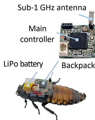
Figure 3: Electronic “backpack” (wireless stimulator) and cyborg insect
