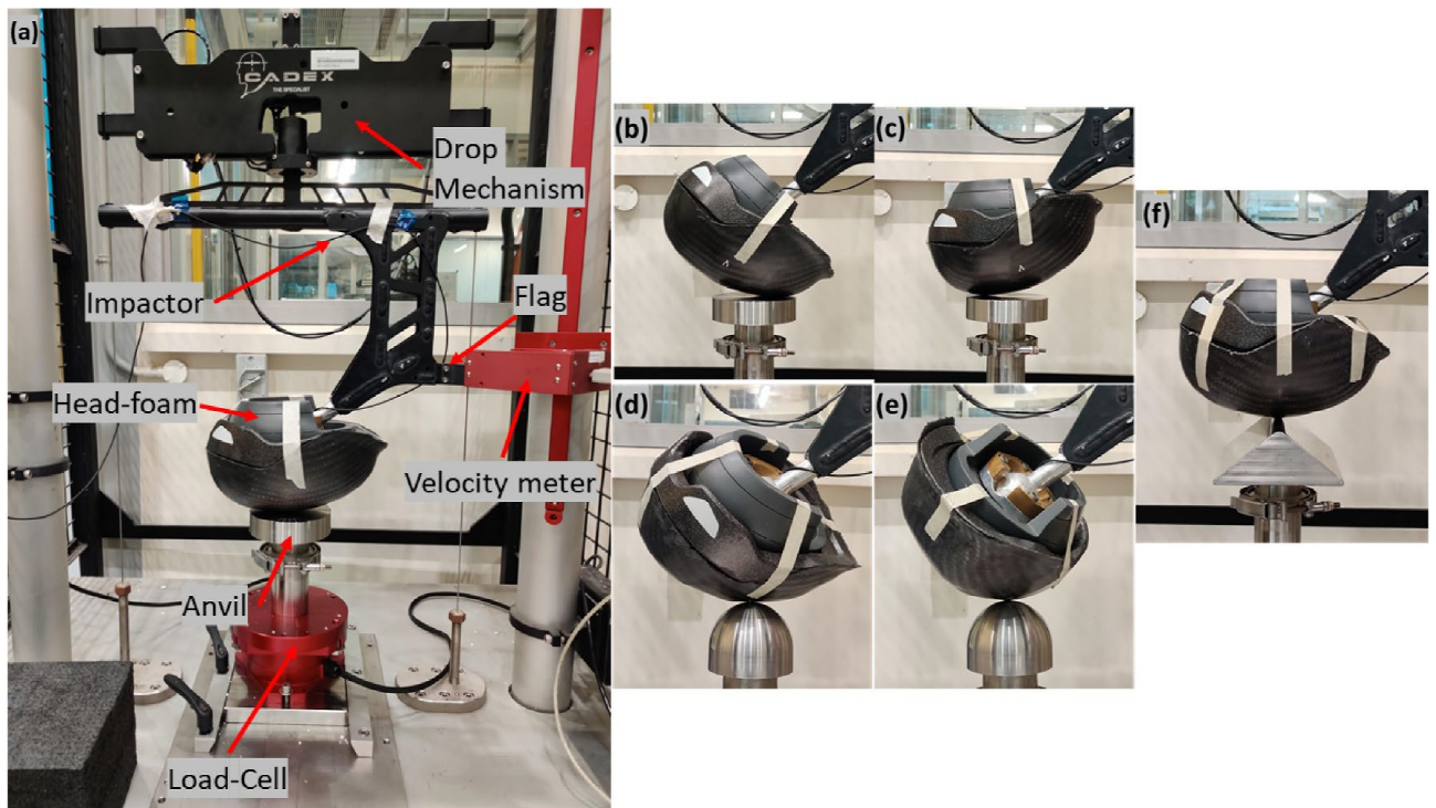
Image 2: The helmet prototype is attached to an impactor arm (a) which drives it down onto a variety of different anvil types at high speeds to test its durability. Tests (b) and (c) show a flat anvil surface, (d) and (e) show a hemispherical anvil, and (f) is a curbstone anvil test.
