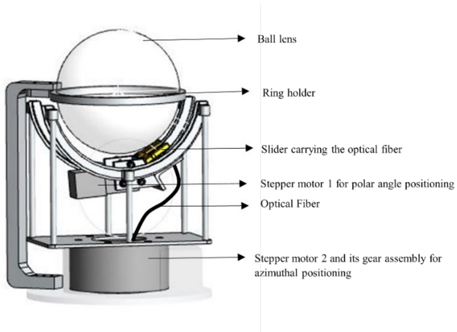
Image 1: Design of the ‘smart’ device to harvest daylight
