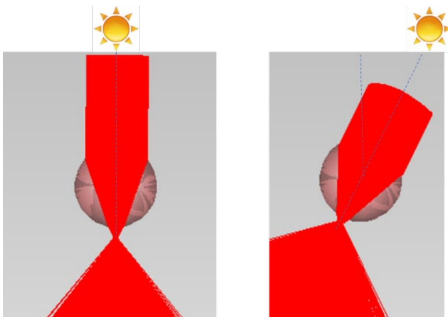
Image 2: Shifting of focused light spot under the ball, in accordance with sun’s position in the sky
