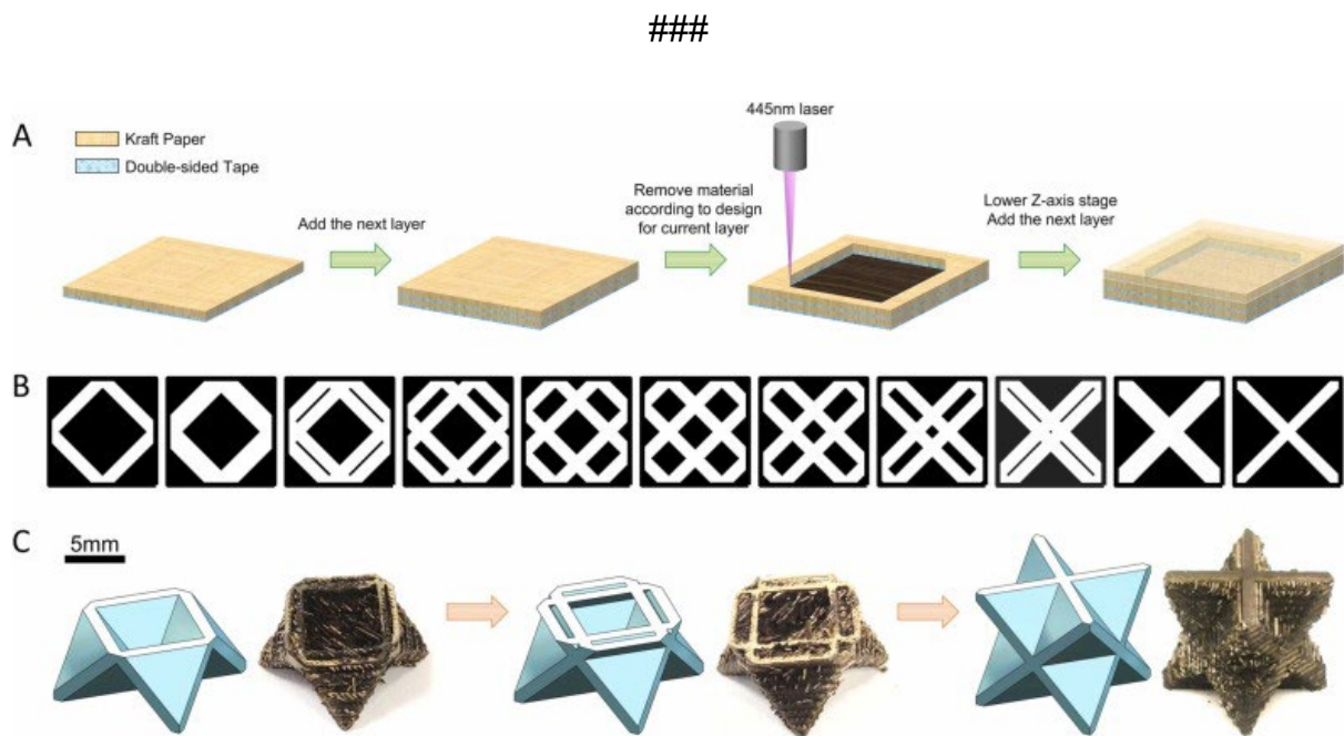
Figure 1: Illustration of the process to convert kraft paper into anodes, developed by NTU Singapore. The structures were turned into carbon anodes at high temperatures in a subsequent step.
