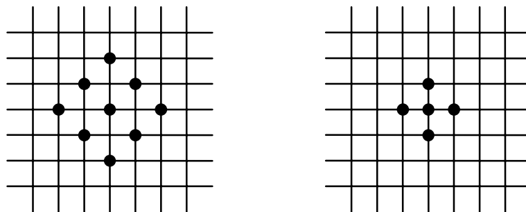
(a) Large diamond search pattern (LDSP) (b) Small diamond search pattern (SDSP)
