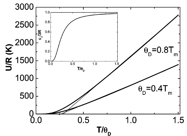
Figure 1. Illustration of the temperature dependence of the reduced specific heat (inset) and its integration with respect to temperature (or the specific internal energy U(T/\theta_D) ). The melting temperature is chosen to be 1000 K for illustration purposes. For consideration of a single bond, one has to divide the values by the atomic coordination number (CN) z . The c_v(T/\theta_D) and U(T/\theta_D) are sensitive to the Debye temperature.
